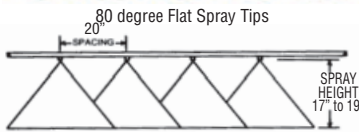
80 & 110 degree FLAT SPRAY TIPS (Based on 20" spacing)
